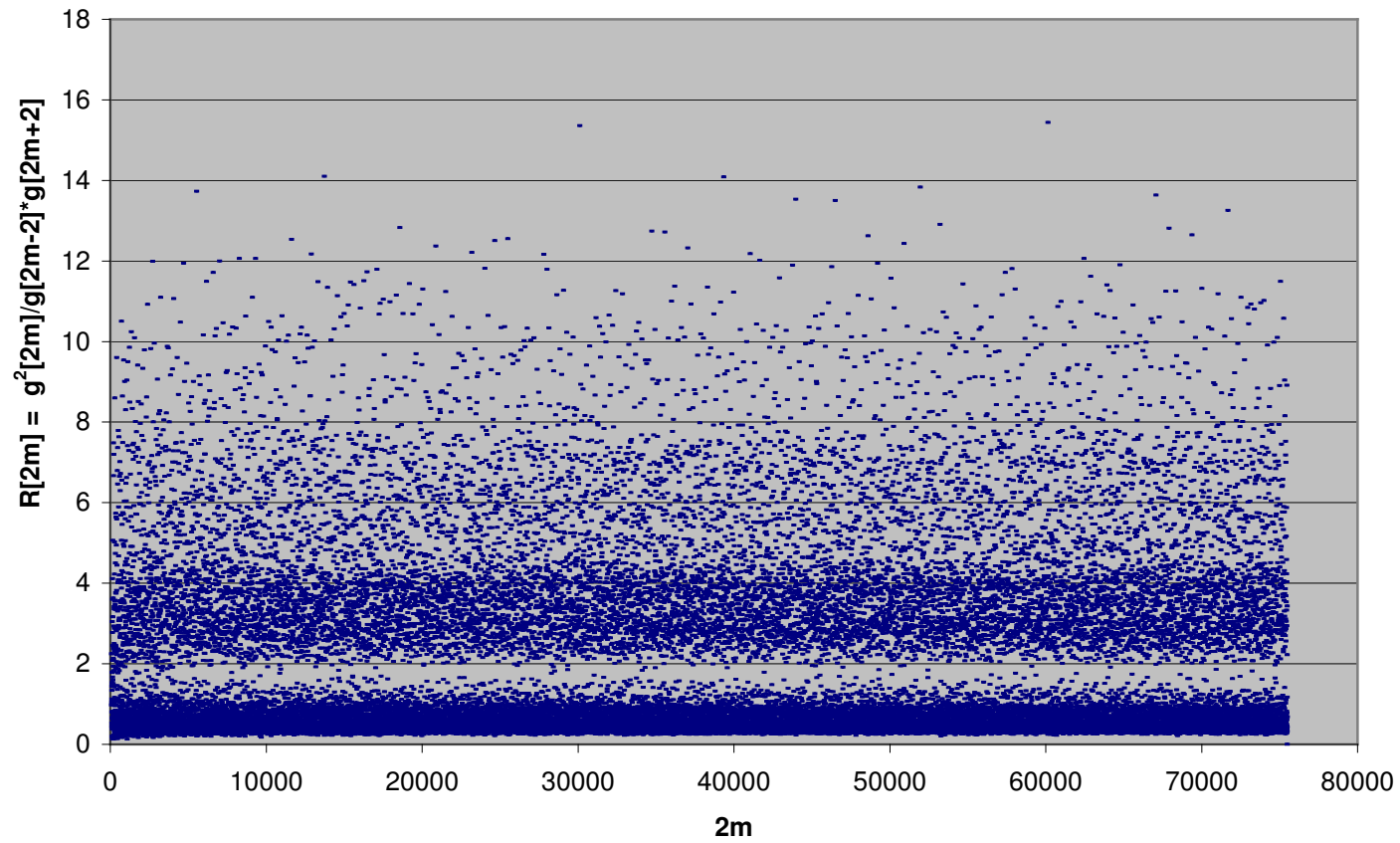
Fig. 1 Ratio of Goldbach Partitions for an even number 2m The ratio R[2m] = g^2[2m]/g[2m-2]*g[2m+2]
